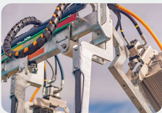
FULL 90° BREAKAWAYS
